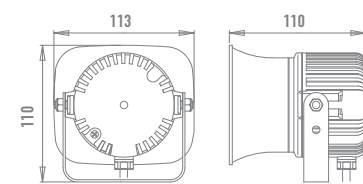
LOUDSPEAKER - NSC
