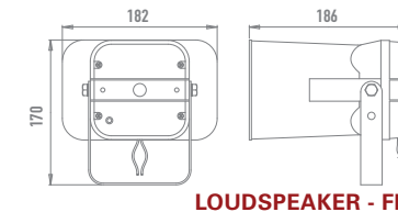
LOUDSPEAKER - FB
