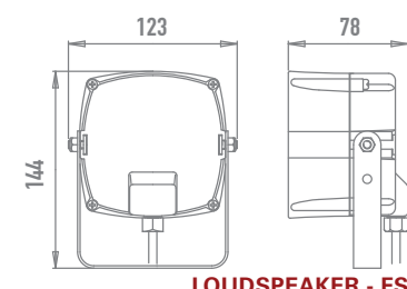
LOUDSPEAKER - FS
