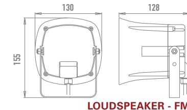
LOUDSPEAKER - FM
