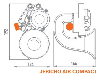
JERICHO AIR COMPACT
